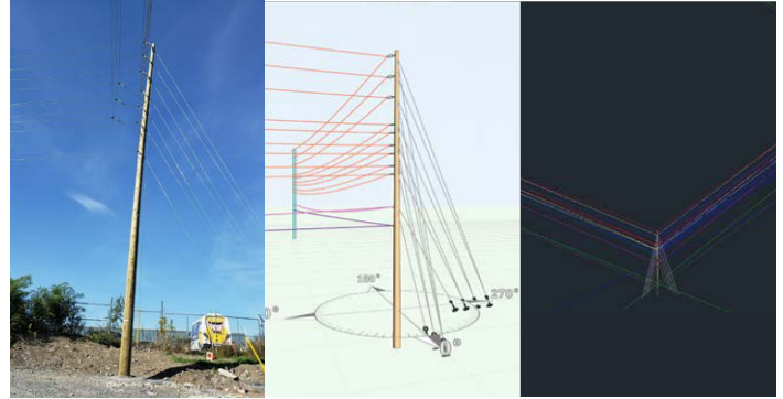
SPIDAlcalc simplified the design analysis process in the electrical services sector while offering an accurate 3D view and showcasing complex features for analysis.
